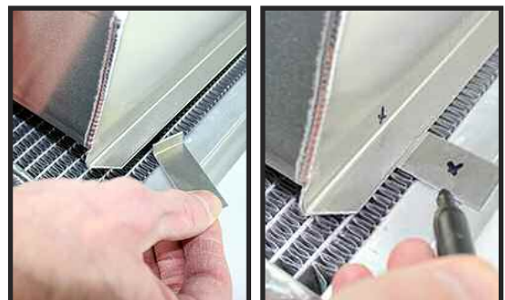
PHOTO 15: Insert & Mark location.
