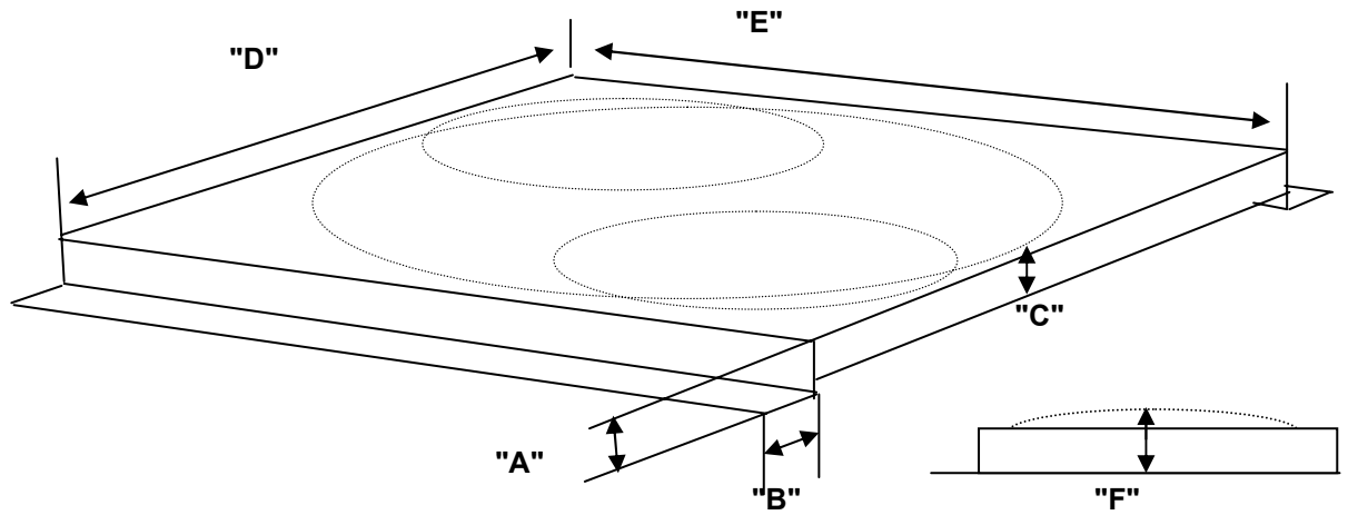
Fan Shroud Measurements
