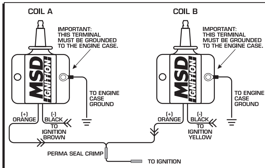
Figure 2 Dual Coil System.
