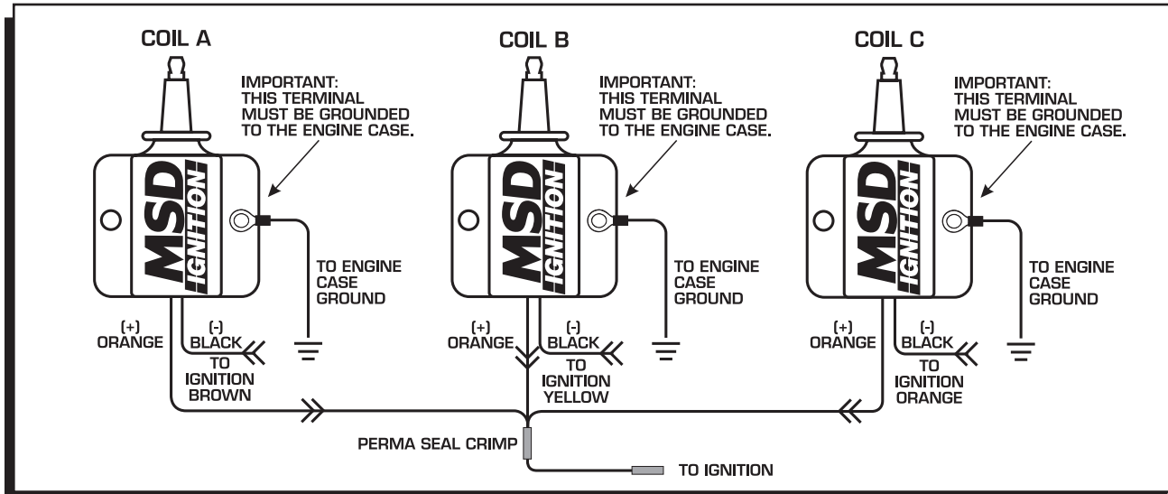
Figure 3 Triple Coil System Used with PN 42351 Ignition.
