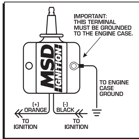
Figure 1 Single Coil System.
