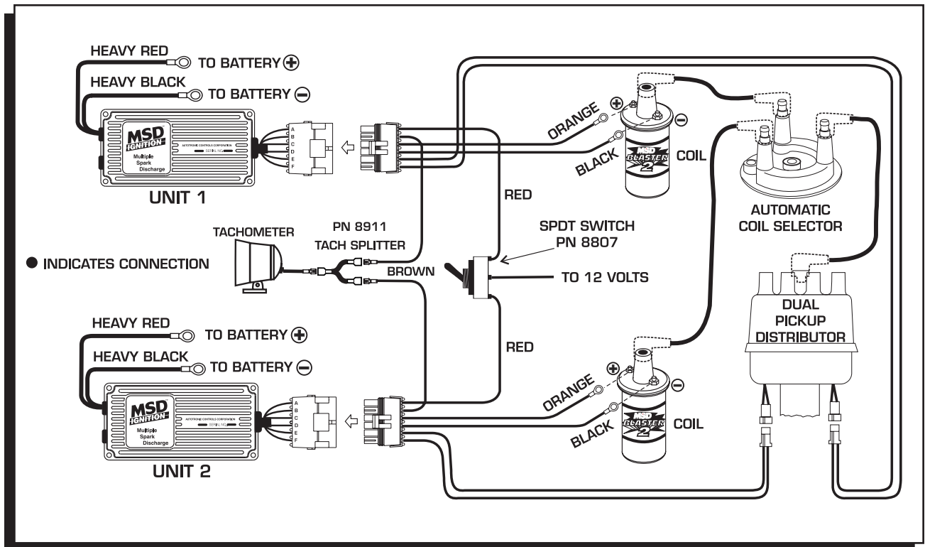
Figure 4 Two MSD 6 Series and Coils with a Dual Magnetic Pickup Distributor.
