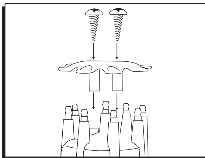
Figure 10 Installing the Wire Retainer
