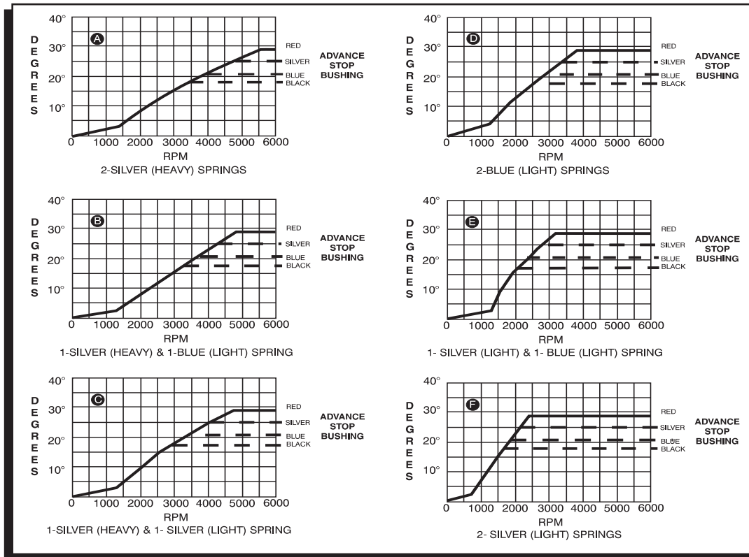
Figure 4 Advance Curves.
