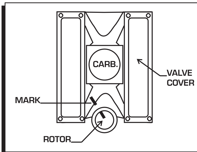
Figure 8 Marking the Rotor Location.
