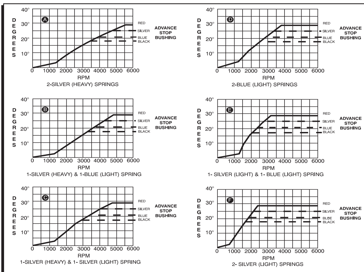
Figure 4 Advance Curves.
