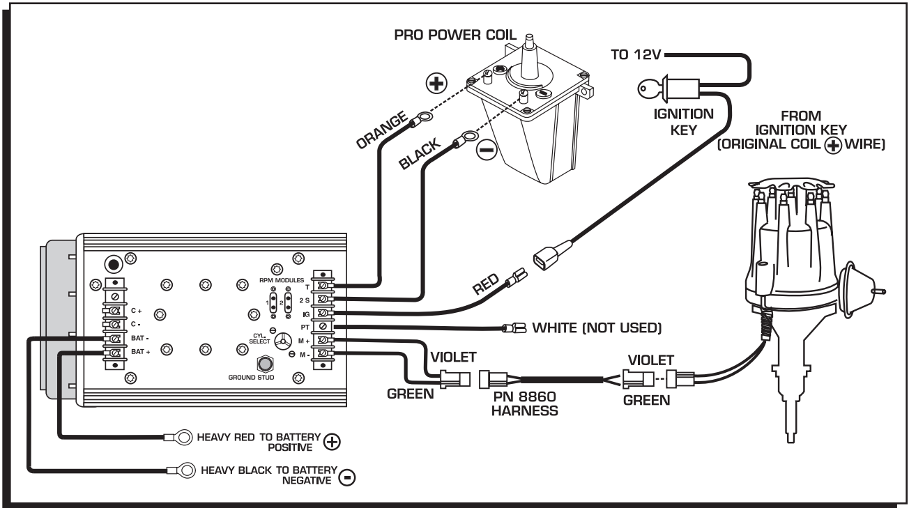
Figure 15 Wiring to an MSD 7-Series Ignition Control.
