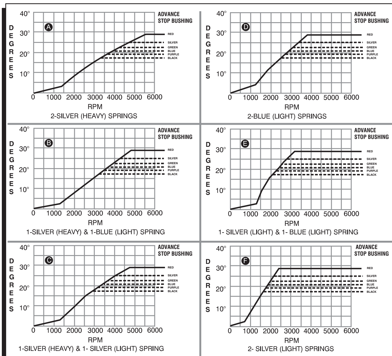
Figure 4 Advance Curves.
