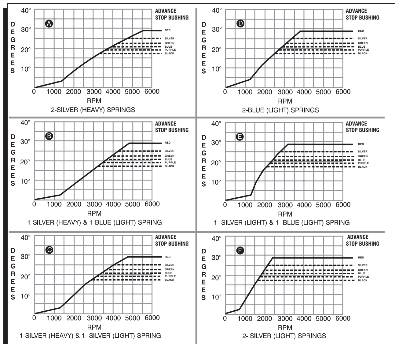
Figure 4 Advance Curves.
