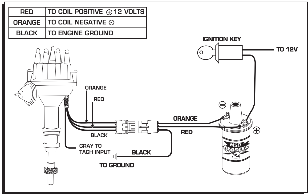
Figure 13 Wiring the Ready-to-Run Ford Distributor.
