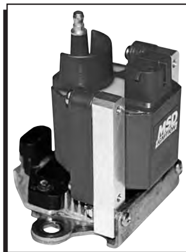
Figure 3 LT1 Assembled.
