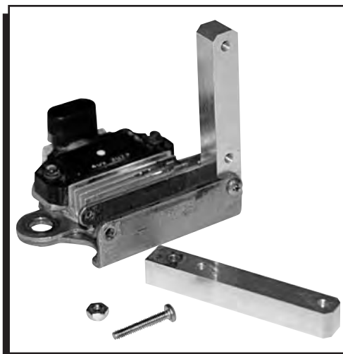
Figure 2 LT1 Brackets.
