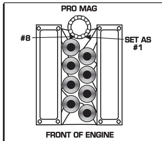
Figure 4 Recommended Chevrolet Installation Position.
