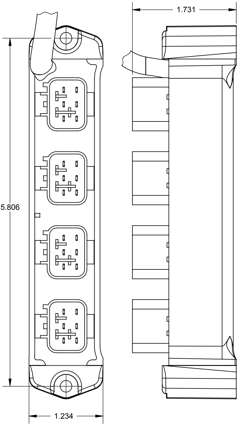
Vertical Mount
