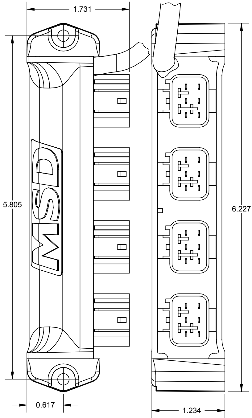
Horizontal Mount
