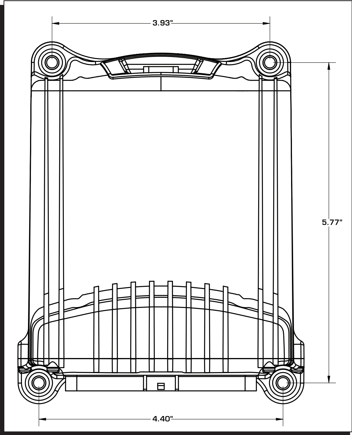
Figure 3 Mounting Template.
