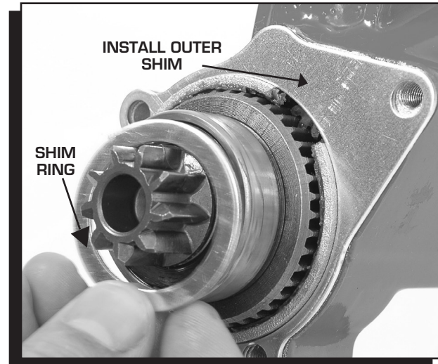
Figure 3 Installing the Pinion Shim Spacers.
