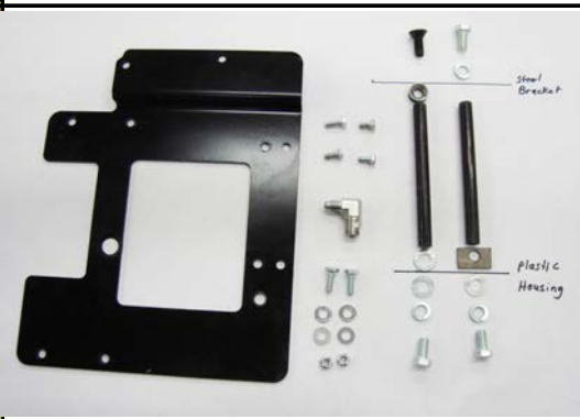
Manifold angle bracket for 2007-2011 Jeep JK
