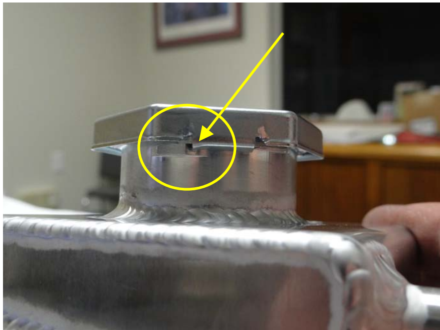
When viewing from bottom side, cap tang should be against billet stop.
