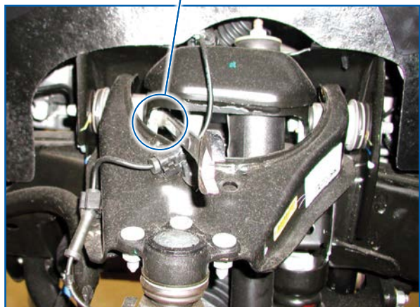
INBOARD LOCATION MAKES ADJUSTMENT DIFFICULT
