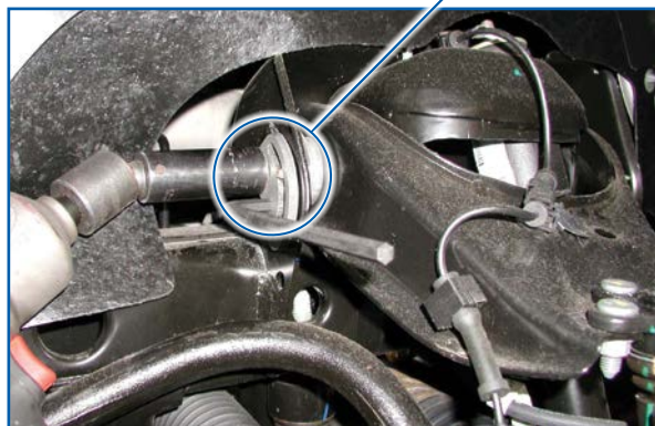
OUTBOARD LOCATION AIDS IN ADJUSTMENTS
