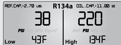
TEMPERATURE/PRESSURE DISPLAY
