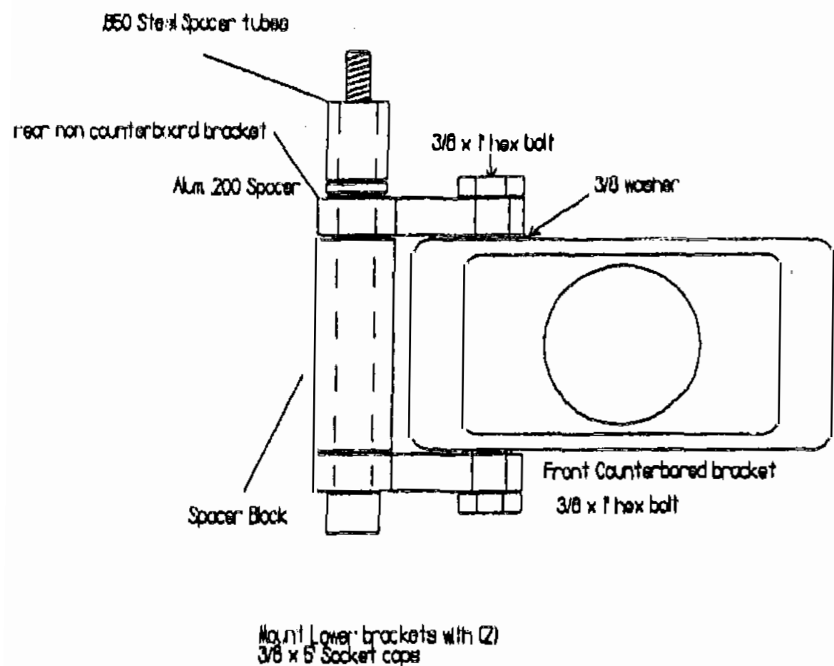
Top view (lower) Brackets Using Standard G.M. Sag. Pump
