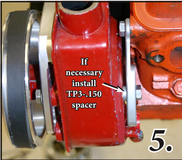
Photo 5. Install the Rear Support Bracket (22026-C) to the outer head bolt using (1) \frac{3}{8} - 16 x \frac{1}{2} " Hex Head Bolt (S308)
