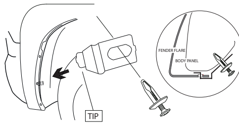
Lever Clip with Plastic Fastener
