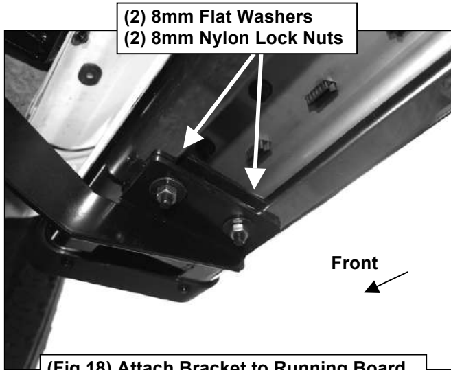
(Fig 18) Attach Bracket to Running Board
