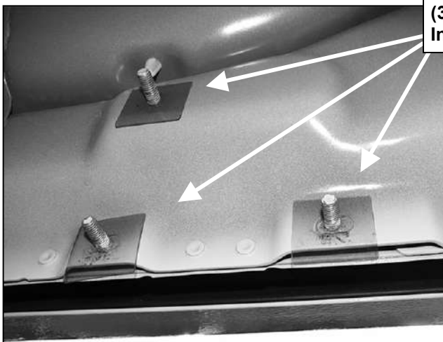
(Fig 3) Thread Plastic Washers onto all mounting studs. Passenger side rear pictured
