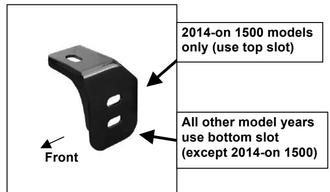
(Fig 2A) Driver/left Front Bracket
