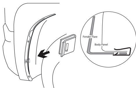
Push U-Clip
