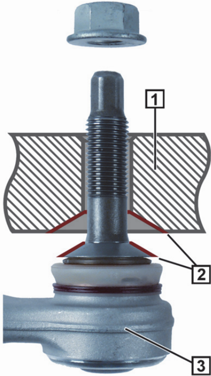
Fig.1: Rear axle control with cone seat (2)
