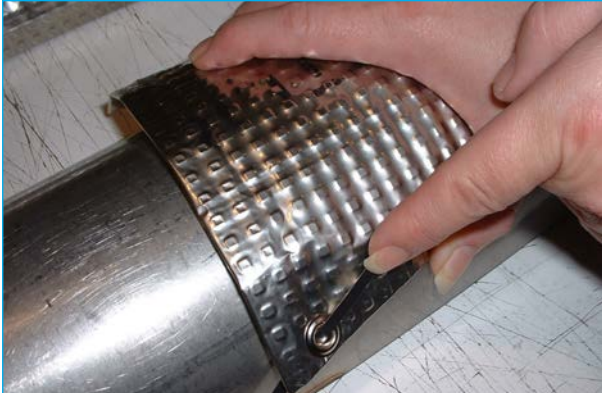
Strap Shield to Exhaust with Wire or Metal Straps
