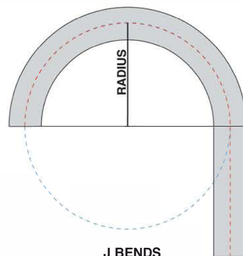
J BENDS
