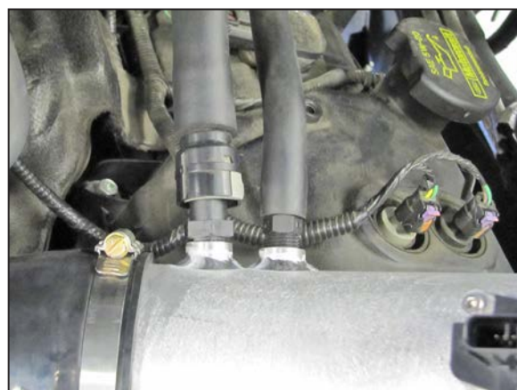
19. Connect the EVAP vent line and crank case vent lines to the fittings installed into the K&N® intake tube.
