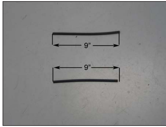
12. Cut the provided edge trim into two 9" sections as shown.
