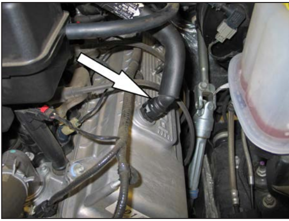
7. Disconnect the crank case vent tube from the valve cover port.
