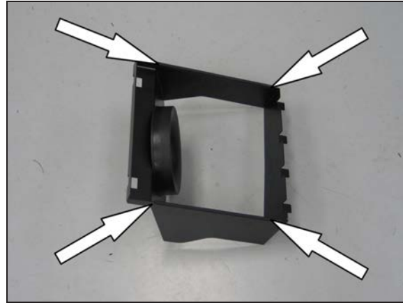
13. Install the cut edge trim onto the bottom of the heat shield as shown.
