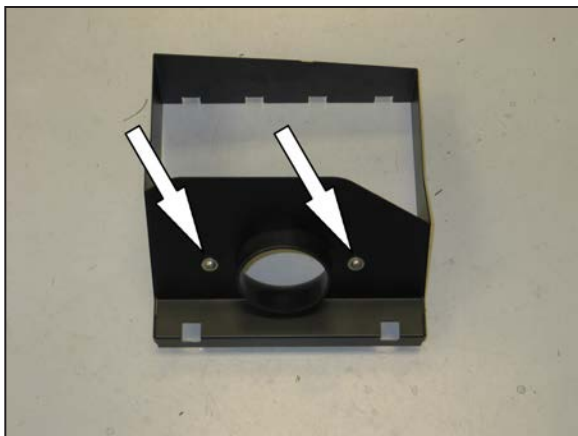
11. Install the K&N® filter adapter into the heat shield as shown and secure with the provided hardware.
