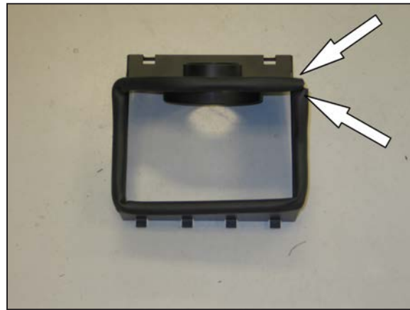
14. Install the provided "Top bulb" edge trim onto the top off the heat shield as shown. NOTE: Some trimming of the edge trim will be necessary.
