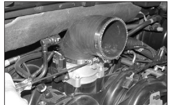
17. Install the 90° silicone hose and hose clamps onto the throttle body as shown but do not tighten completely at this time.
