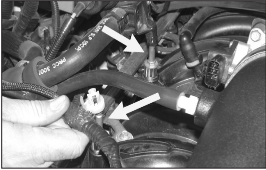
8b. Re-install the heater control valve and wiring harness mounting clips onto the airbox mounting studs as shown.
