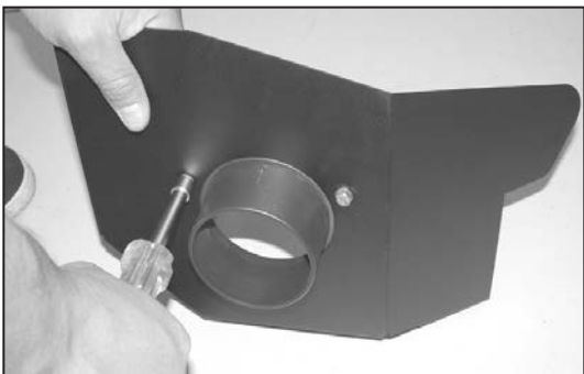
12. Apply the provided thread locker onto the provided hardware and secure the filter adapter onto the heat shield as shown.
