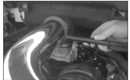
17a. On vehicles equipped with the brake booster vent line install the K&N® intake tube into the silicone hose at the throttle body. Align the brake booster vent line to the K&N® intake tube as shown and place a mark for drilling location.
