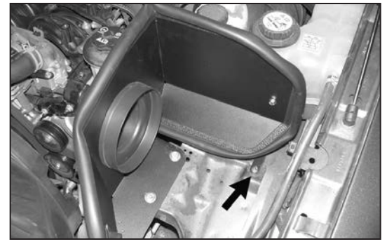
16. Install the heat shield into the vehicle and secure the "L" bracket to the threaded hole on the inner fender using the provided hardware as shown but do not tighten at this time.
