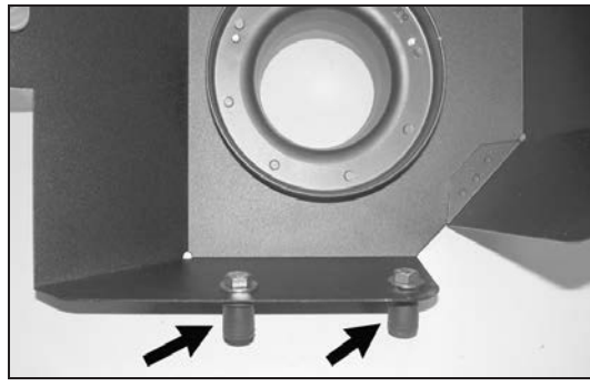
13. Install the provided rubber inserts, hex bolts and washers onto the heat shield as shown, but do not tighten at this time.
