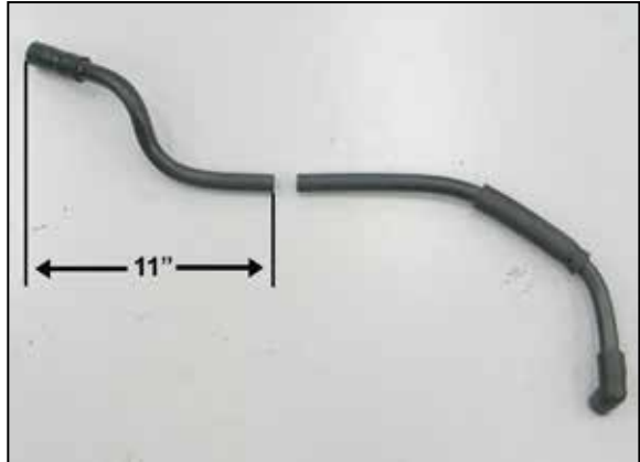
8. Measure 11" from the air filter end of the crank case vent tube and then trim the crank case vent tube as shown.
