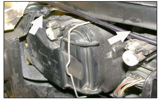
22. Remove the two upper plastic rivets from the inner plastic headlight cover as shown.
