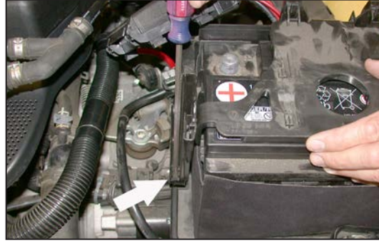
17. Depress the two lower release tabs on each side of the secondary battery cover as shown.
