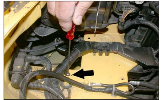
26. Using the provided plastic clamp secure the harness to the inner fender using the provided hardware as shown.
