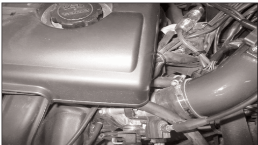
19. Fit the Typhoon tube onto the throttle body, using the original hose clamp removed earlier but don't fully tighten the hose clamp yet!
