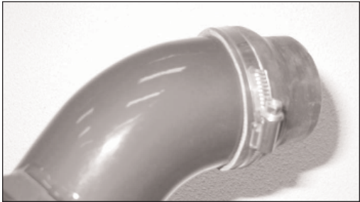
18. Fit the stepped silicone sleeve on the tube using the original hose clamp removed earlier.
