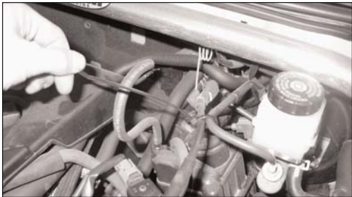
25. Secure the throttle cable to the brake line using the cable tie supplied.
