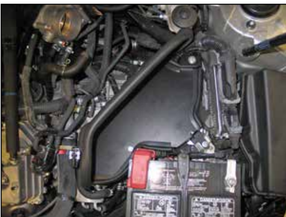
26. Set the heat shield into position and secure with the provided hardware.
