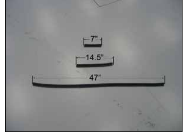
19. Cut the provided edge trim into three sections, the long section is 47" long, the medium section is 14-1/2" long, the short section is 7" long.
