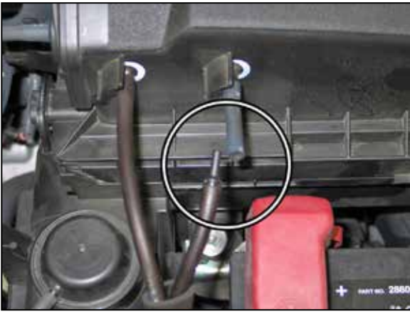
7. Disconnect the vacuum line from the union fitting shown leaving the union installed into the vacuum line attached to the vehicle.
