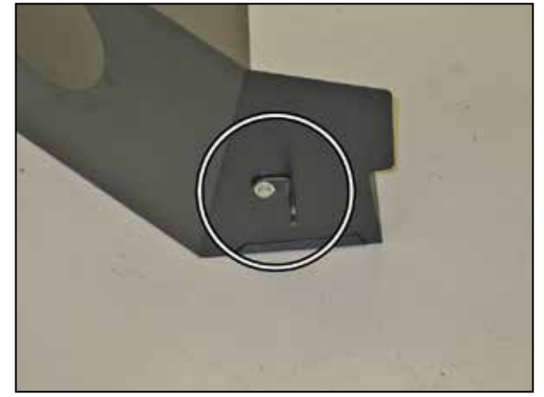
17. Install the heat shield mounting bracket (070066) onto the heat shield using the provided hardware.
