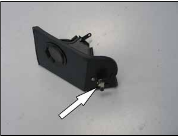
24. Secure the vacuum switching valve to the "L" installed onto the heat shield as shown and then install the provided vacuum caps.
