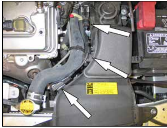
12. Disconnect the vacuum switch electrical connection and then unhook the harness from the fresh air duct.
