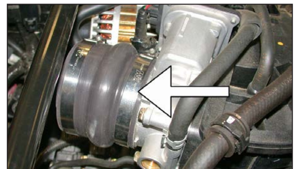
27. Install the silicone hose and hose clamps onto the throttle body as shown.
