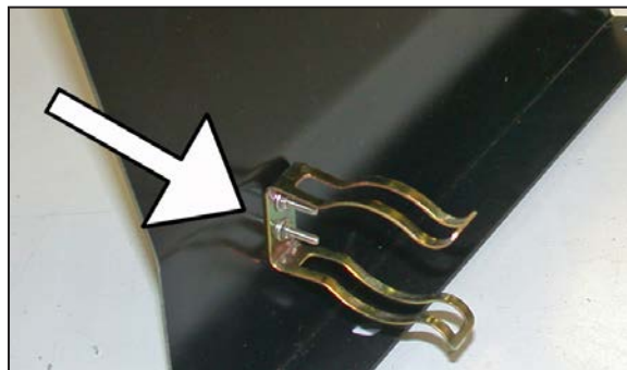
20. Manual trans only, install the canister clip from step 19 onto the heat shield using the provided hardware.
