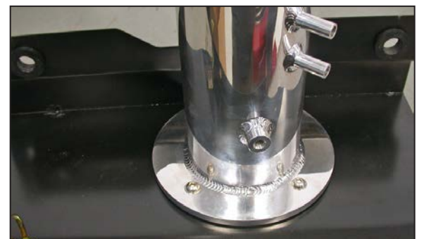
25. Install the K&N® intake tube onto the heat shield and secure with the provided hardware as shown.
