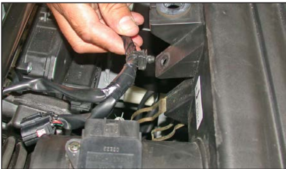
12. Using a pair of pliers, unclip the wire harness from the air cleaner assembly as shown.
