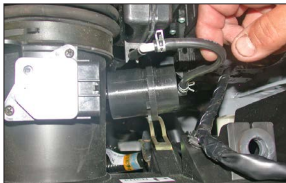
5. On manual transmission vehicles, remove the vacuum canister from the clip on the side of the airbox assembly.
