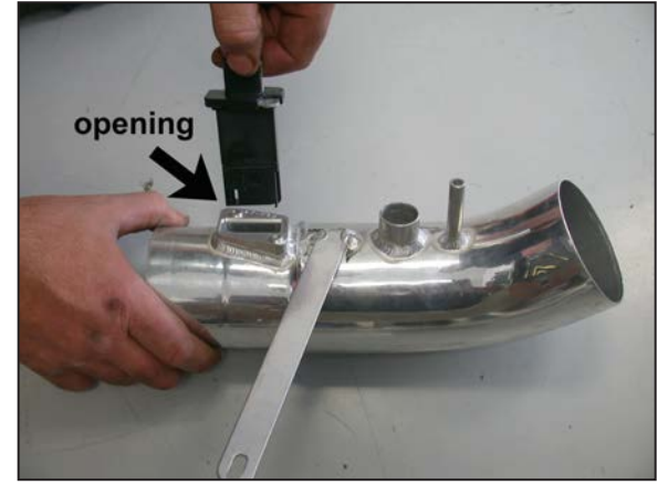
17. Install the mass air assembly into the intake tube and secure with the provided hardware. NOTE: Be sure to install with the opening of the mass air sensor towards the filter end of the tube as shown.
