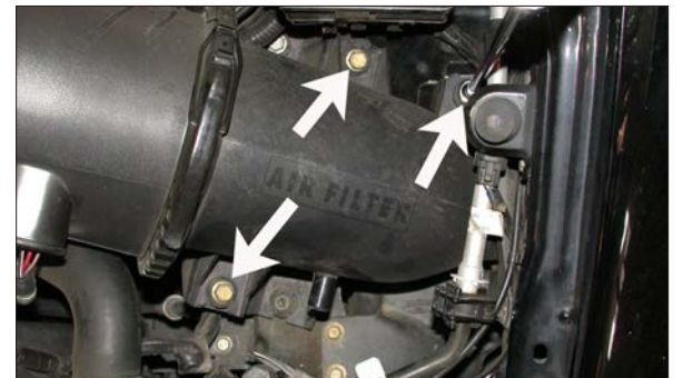
7. Loosen and remove the three bolts that secure the air cleaner assembly as shown.
