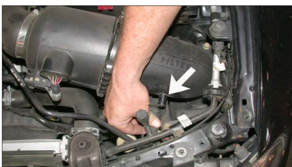
3. Disconnect the crank case vent hose from the stock air cleaner assembly as shown.
