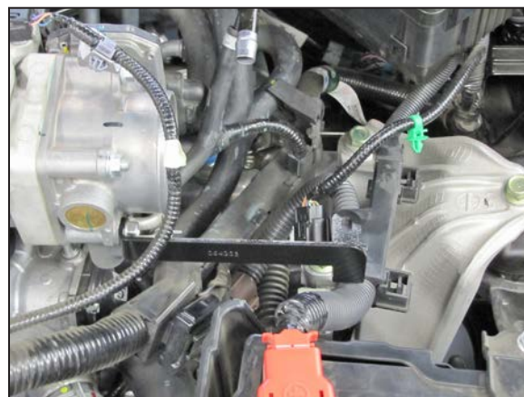
14. Install the provided tube mounting bracket (064302) onto the throttle body and secure with the factory bolt removed in the previous step.
