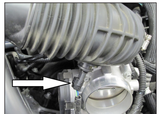
6. Lift up the intake tube, disconnect the inlet air temperature electrical connection then remove the intake tube from the vehicle.
