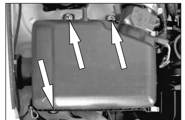
5. Loosen the three bolts that retain the air box assembly.
