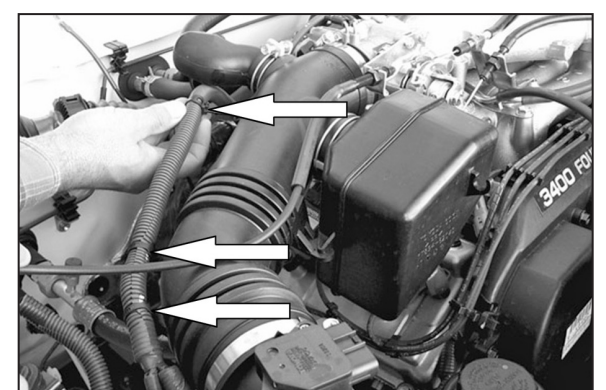
6. Remove the three clips that hold the electrical loom to the intake tube as shown.
