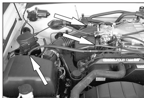
3. Disconnect the three hoses from the air box resonator and intake hose. NOTE: On 03 models, vehicles come equipped with only two vacuum lines.
