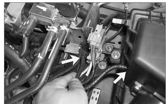
9. Remove vacuum line from bypass solenoid as shown. NOTE: It's the vacuum line that connects to the airbox lid.
