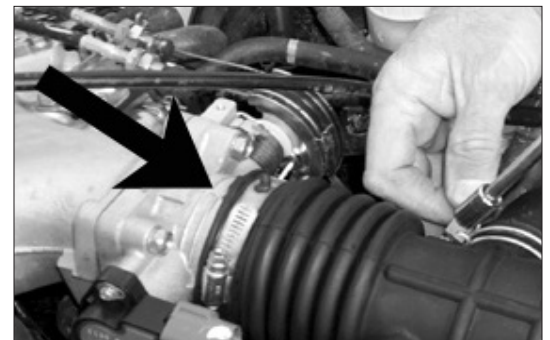
8. Loosen clamp at the throttle body using an 8mm socket.
