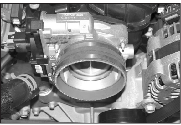
22. Install the silicone hose (08755) onto the throttle body and secure with the provided hose clamp as shown.
