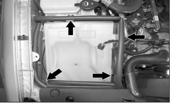
21. Install the heat shield onto the washer reservoir and secure the heat shield and mounting bracket with the provided hardware. NOTE: Be sure to place the mass air sensor wiring harness through the notch in the heat shield before tightening.
