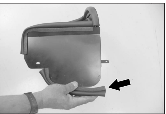
16. Install one of the 10" pieces onto the bottom of the front wall as shown.
