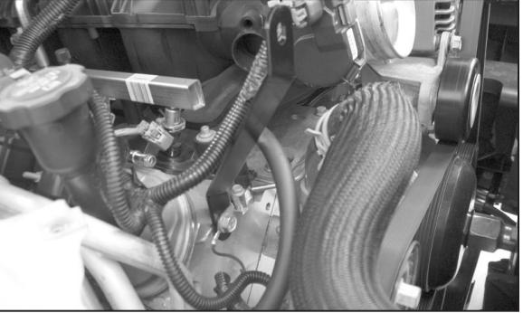
20. Using the bolt removed in step #19, secure the tube mounting bracket and ground strap to the cylinder head in the same location the bolt was removed from.
