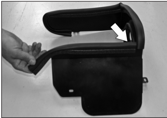
15. Install the 13" long edge trim onto the top of the front wall of the heat shield as shown.
