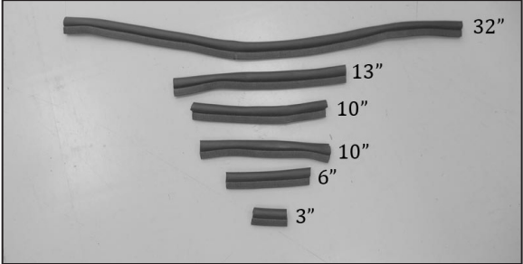
13. Cut the supplied long edge trim into lengths of 32", 13", 6", 3" and 2 pieces at 10".
