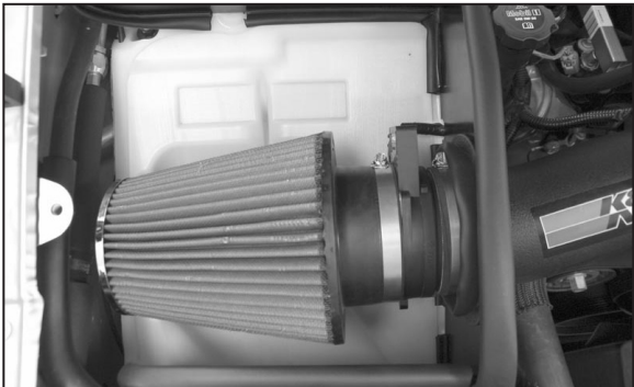
29. Install the K&N® Air Filter onto the mass air sensor and secure with the provided hose clamp as shown. RF-1032DK is available to purchase separately.
