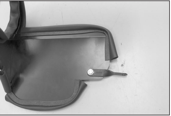
18. Install the mounting bracket onto the heat shield with the provided hardware as shown. NOTE: The slotted end of the bracket will fasten to the heat shield.
