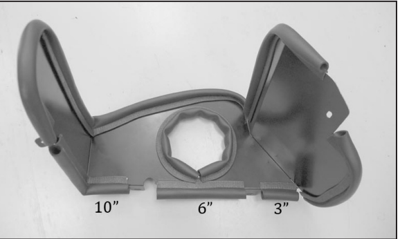
17. Install the remaining 10", 6" and 3" edge trim to the bottom of the heat shield as shown.
