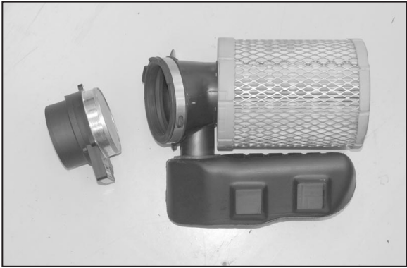
11. Loosen the hose clamp, which secures the mass air sensor to the filter assembly, and then remove the mass air sensor as shown.
