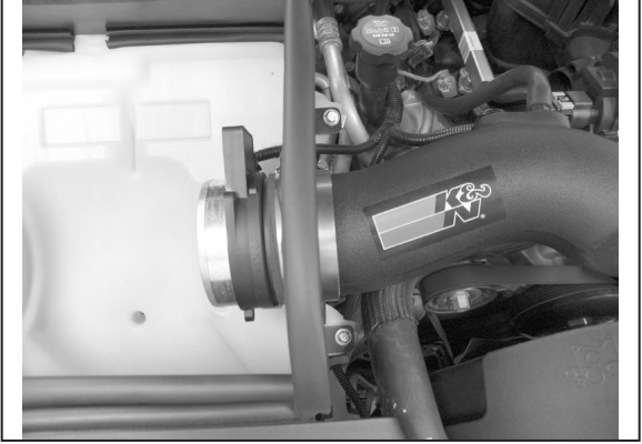
27. Install the mass air sensor assembly onto the intake tube and secure with the hose clamp provided. NOTE: Rotate the mass air sensor so the electrical connection is positioned down towards the electrical connection.
