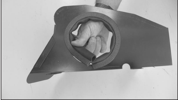
12. Install the 17" piece of edge trim onto the top of the front wall of the edge trim as shown. NOTE: Some trimming of the edge trim will be necessary.
