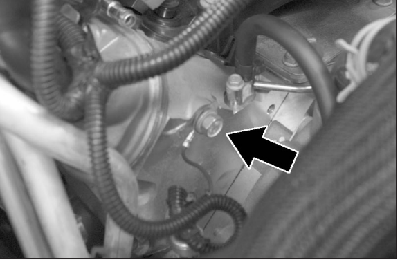
19. Remove the bolt, which secures the ground strap to the cylinder head shown. NOTE: This bolt will be reused.
