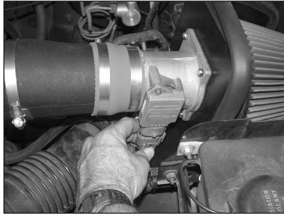
24. Reconnect the mass air sensor electrical connection as shown.
