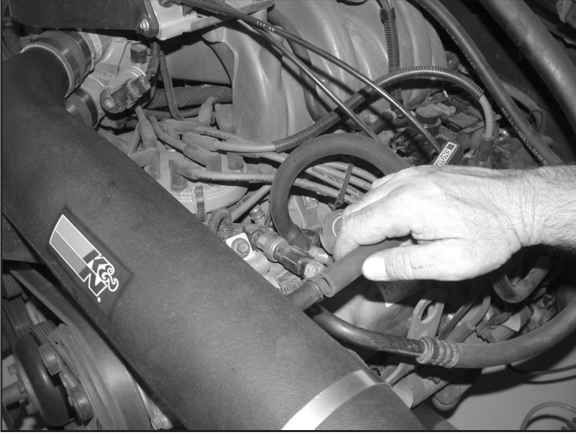
21. Reconnect the crank case vent onto the valve cover, then connect to the intake tube as shown. Trim hose for best fit.
