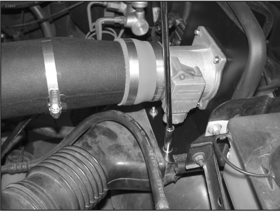
20. Mount the fresh air duct to the heat shield with the provided hardware.
