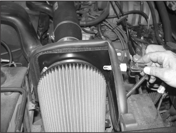
23. Install the temp sensor onto the heat shield then reconnect the electrical connection as shown.
