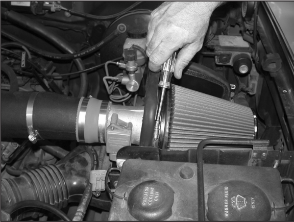
22. Install the Filtercharger to the mass air assembly as shown.
