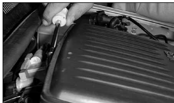
6. Loosen the hose clamp on the intake tube at the throttle body.
