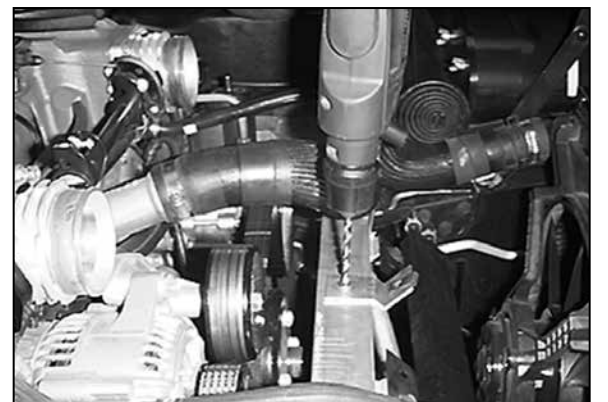
9a. On models equipped with an aluminum crossmember, drill out the rivet that retains the rear air box mounting bracket. Remove the bracket as it will not be used.
