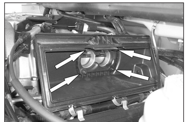
5. Loosen and remove the 4mm nuts that retain the air box base to the throttle body.
