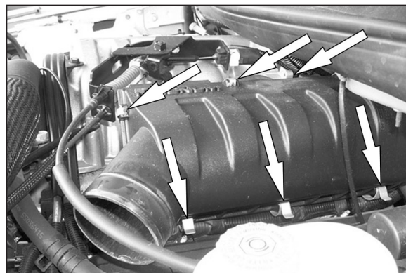
4. Release the 6 clips on air cleaner lid, then remove the air cleaner lid as shown.
