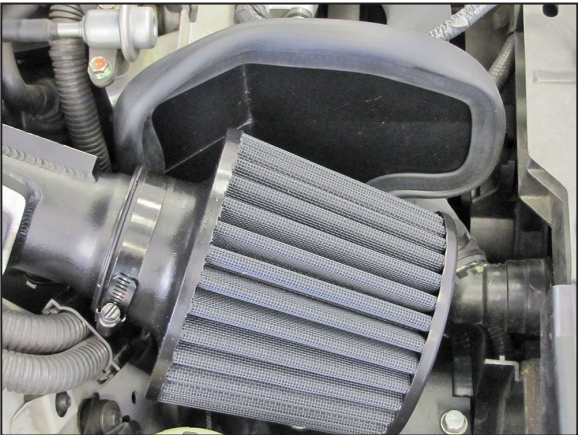
39. Install the air filter onto the intake tube and secure with the provided hose clamp.
